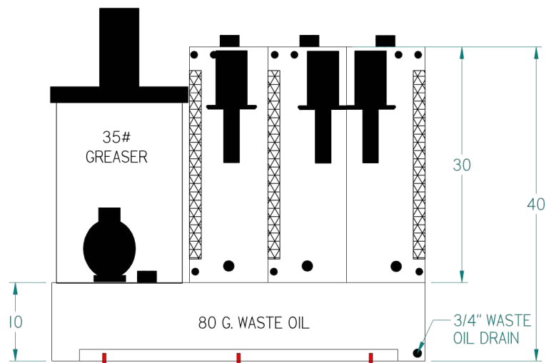
VIEW FROM REAR OF TRUCK
